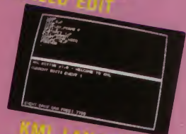
KML LANGUAGE
